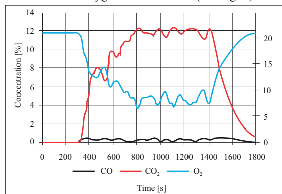
Fig. 1 Gaseous compounds concentration in combustion gas of spruce wood
