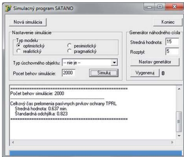
Fig. 2 GUI of SATANO
