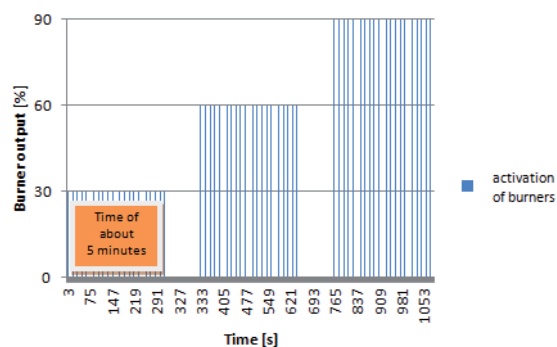
Fig. 4 Activation of gas burners in the course of tests
