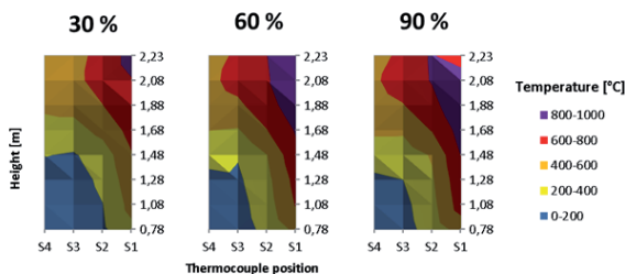
Fig. 6 Median of temperature field distribution in the container longitudinal axis at 30, 60 and 90 percent outputs
