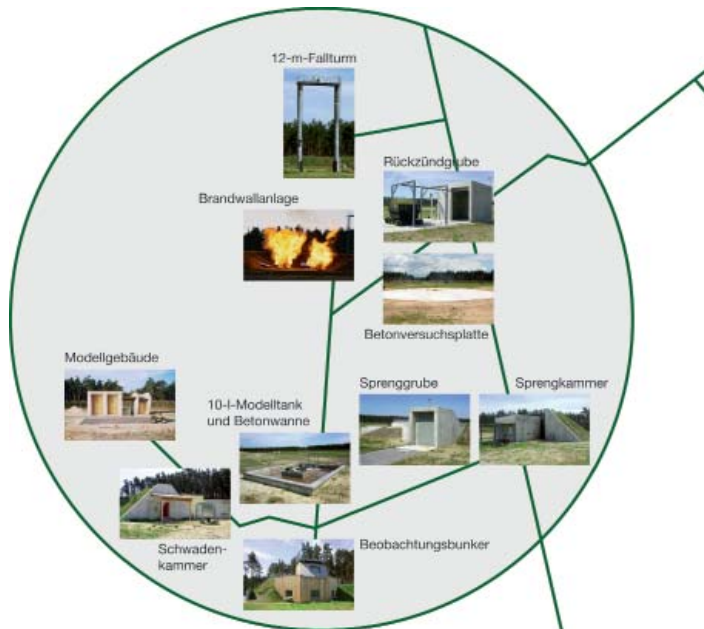
Fig. 7 Test facilities on the blasting area
